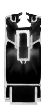
Reversible Saddle Positioned for 1/4" (6 mm) Clearance
